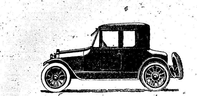
New Model 37A Oldsmobile 3 or 4-Passenger Coupe. 6-Cylinder, 45 H. P., 112 inch Wheel Base. Price $1895 F. O. B. Lansing, Mich.
